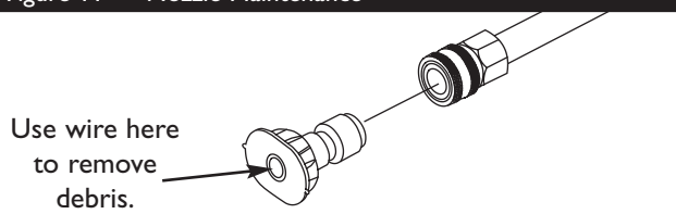
Figure 11 — Nozzle Maintenance
